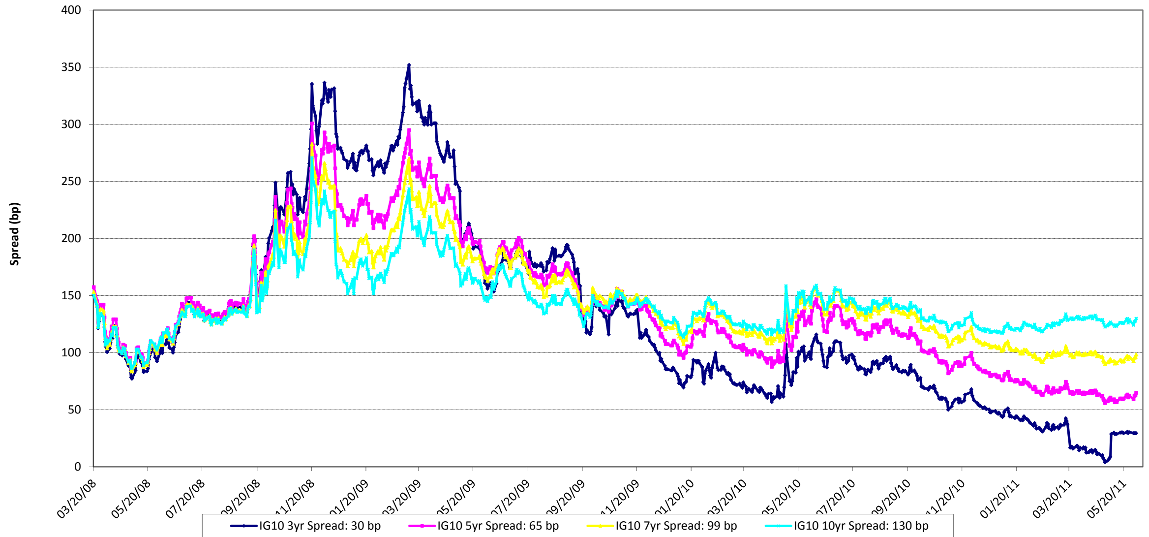
IG10 Spreads
