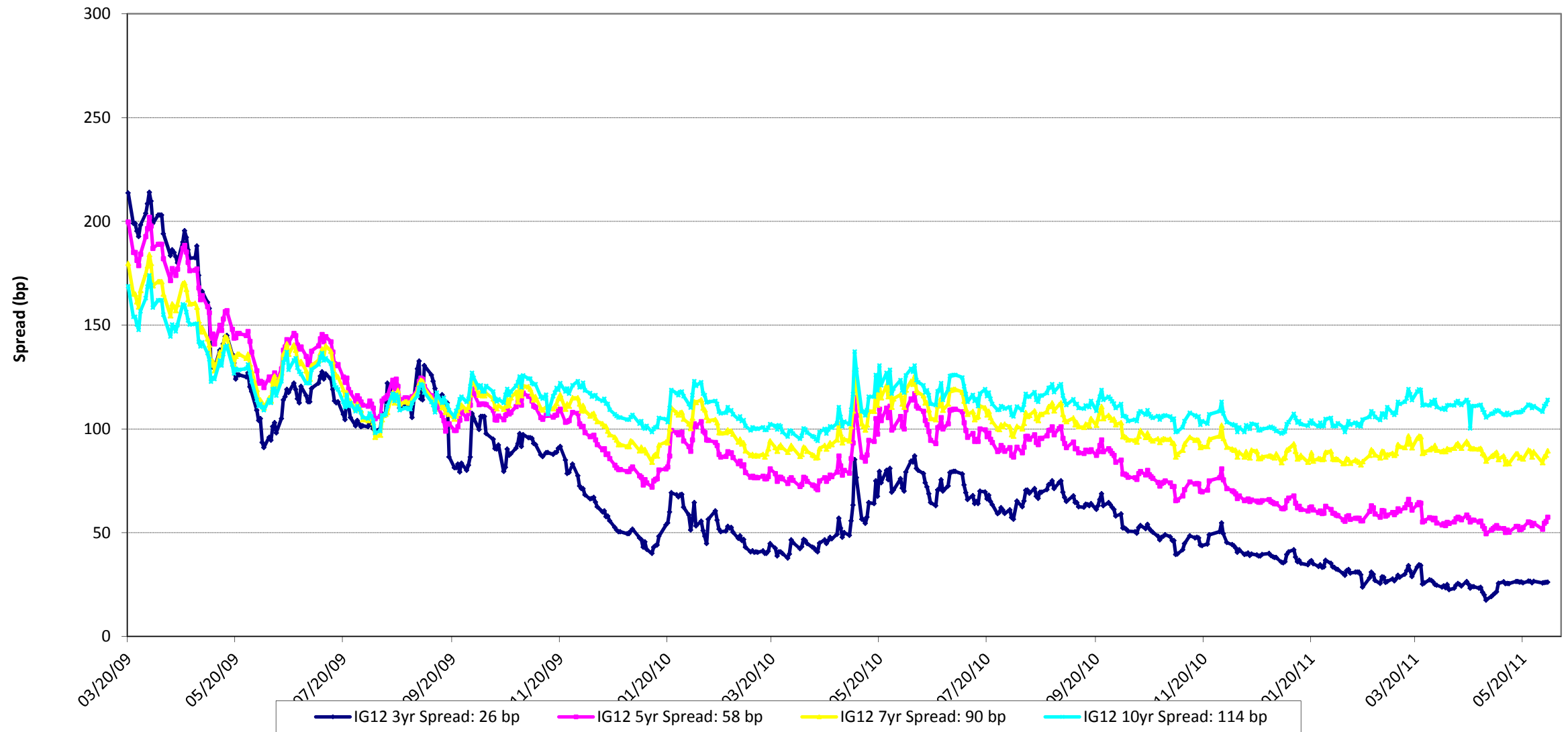
IG12 Spreads
