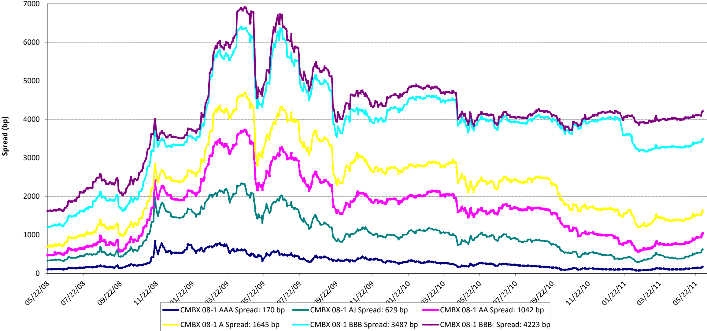
CMBX 08-1 Spreads
