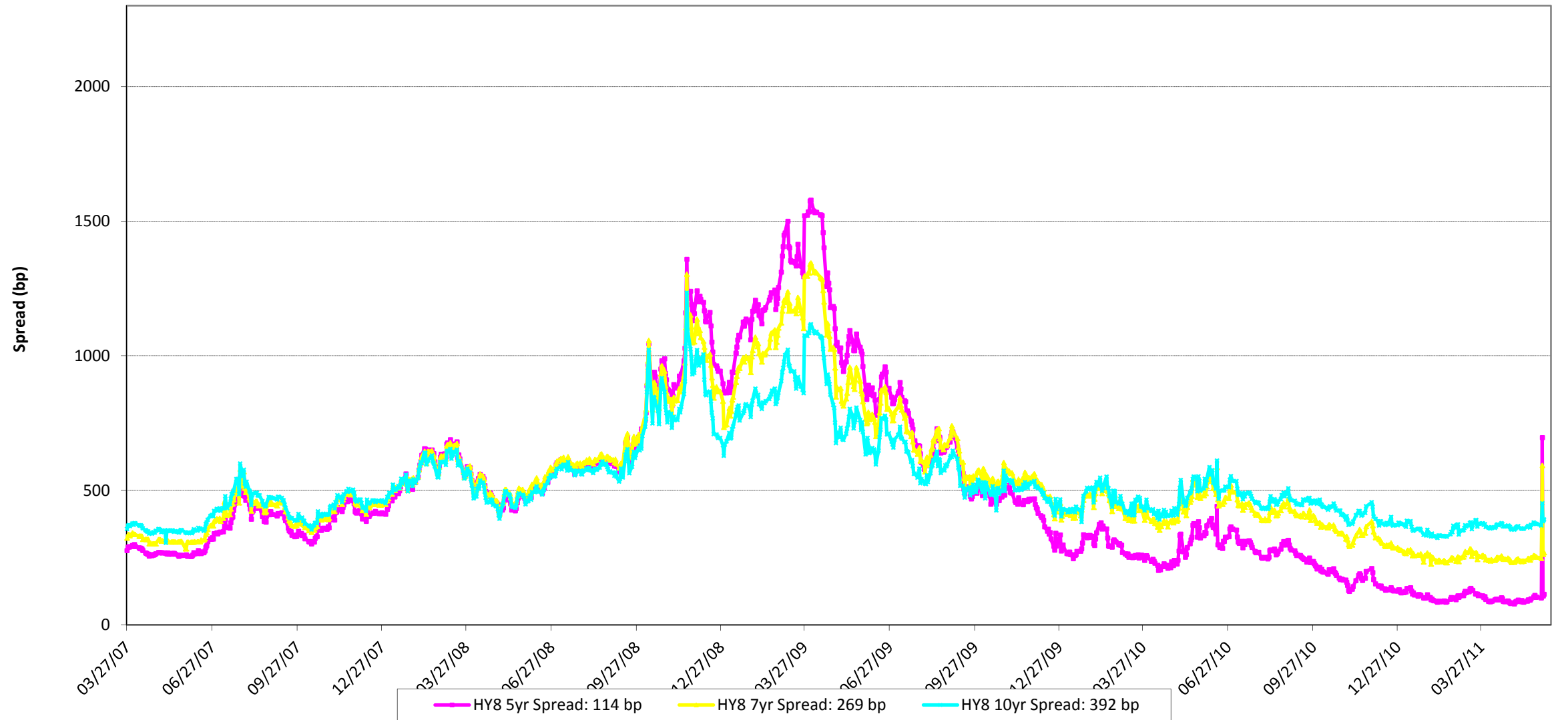
HY8 Spreads
