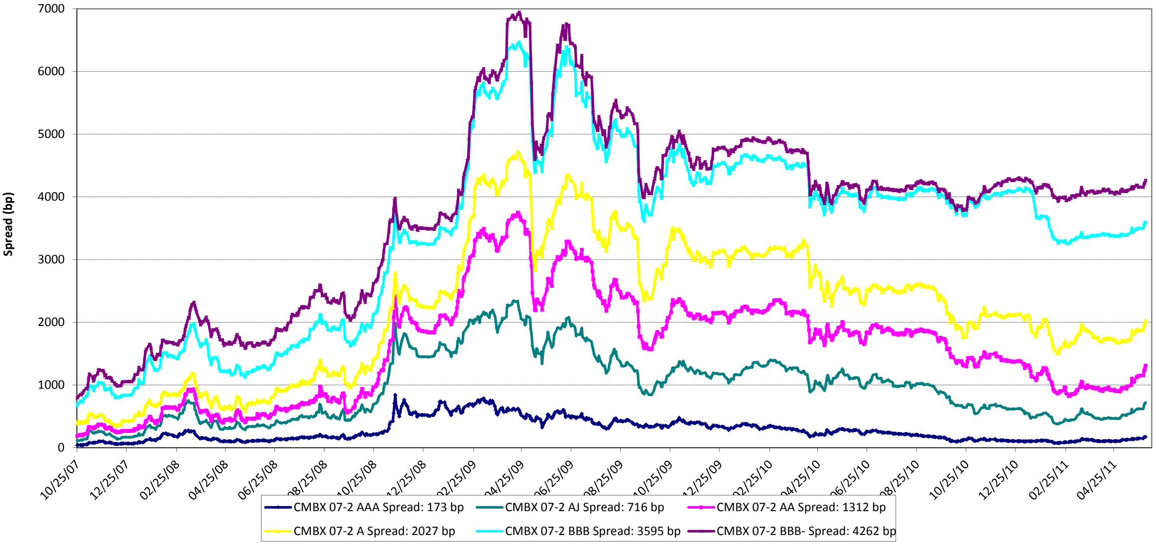
CMBX 07-2 Spreads
