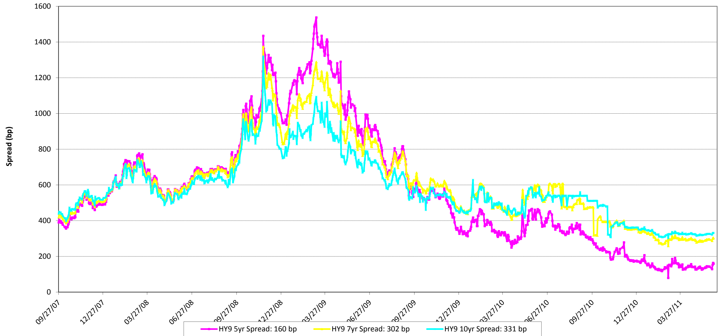
HY9 Spreads
