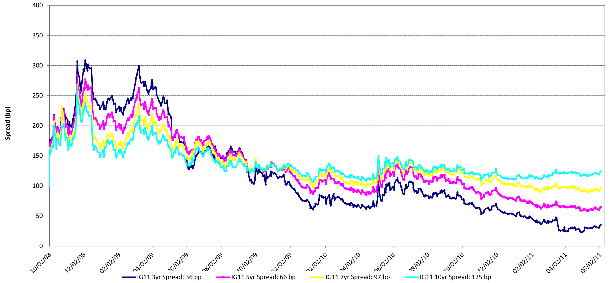
IG11 Spreads
