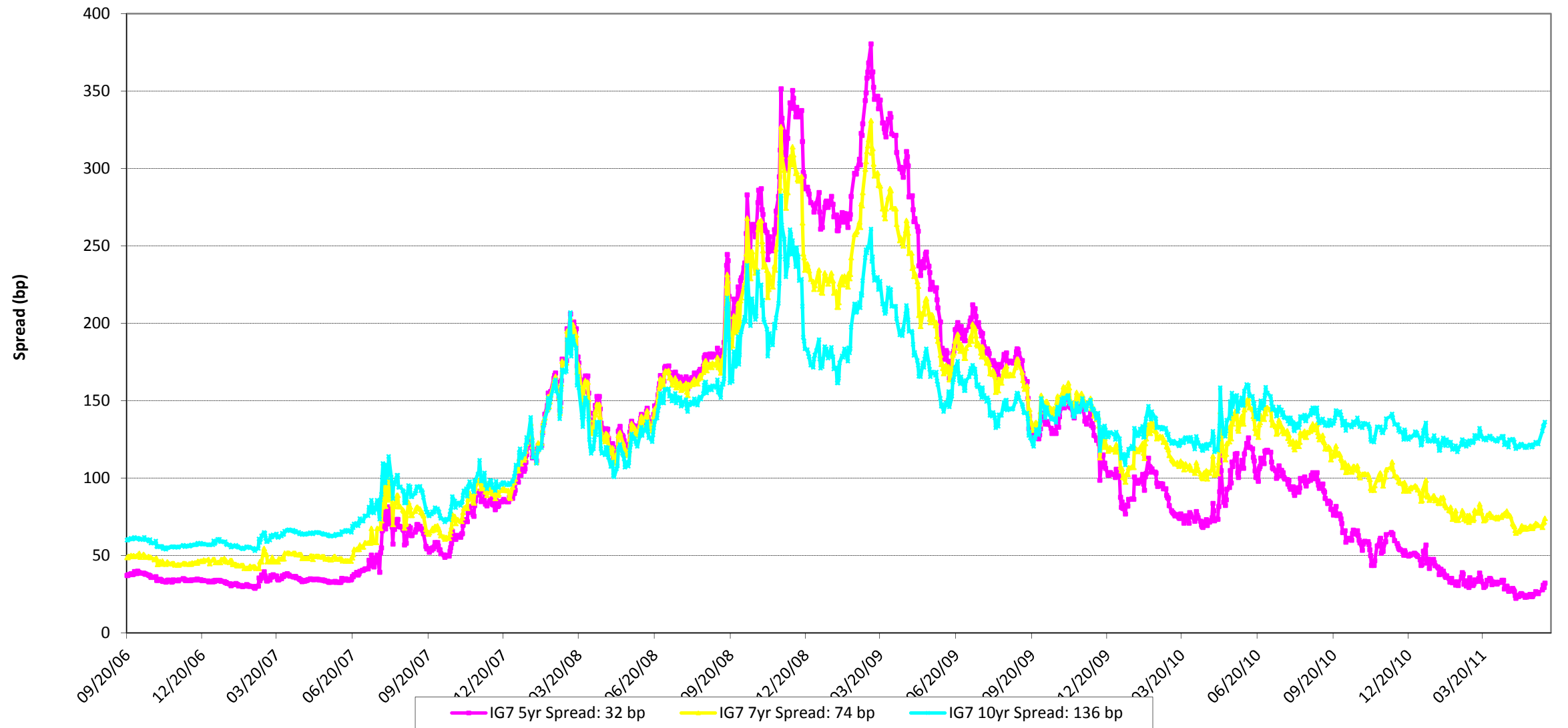
IG7 Spreads
