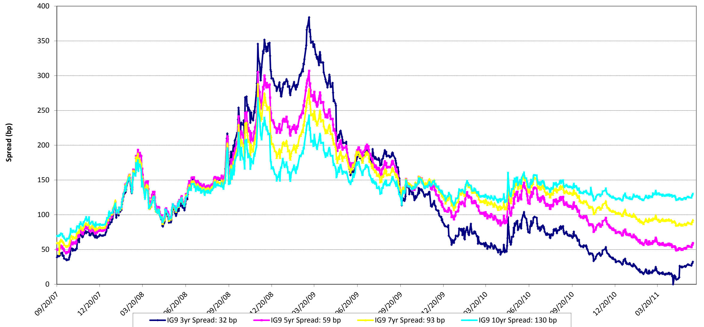
IG9 Spreads
