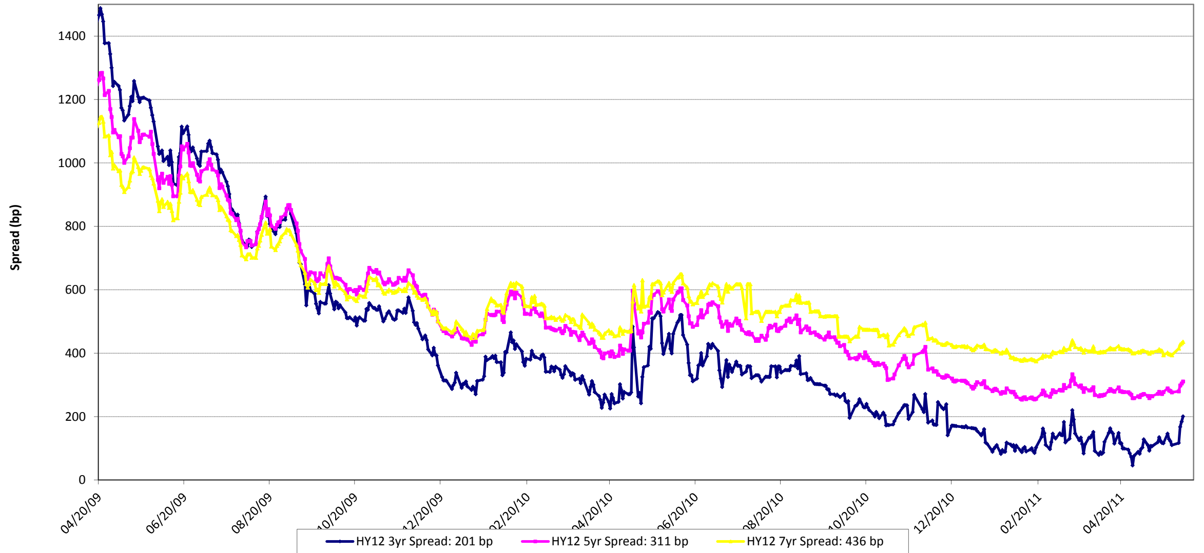
HY12 Spreads
