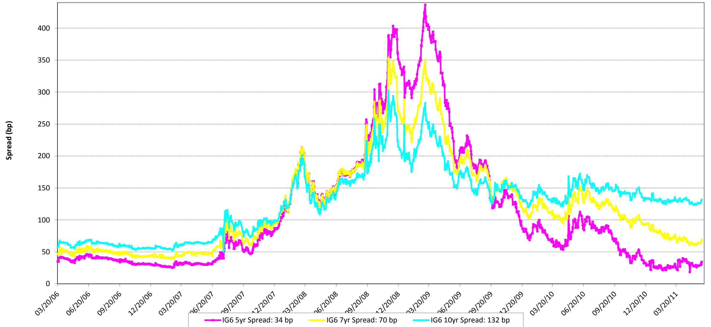
IG6 Spreads
